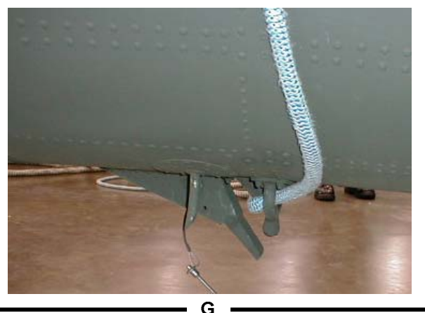
Figure 1. Disabled AH-64A and Recovery Helicopter Rigging
